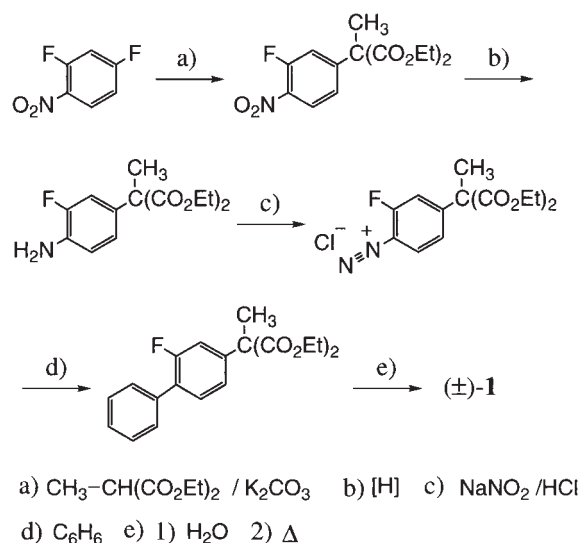
Scheme 1. Industrial preparation of racemic flurbiprofen.
